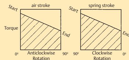
Torque diagram with single acting actuators
